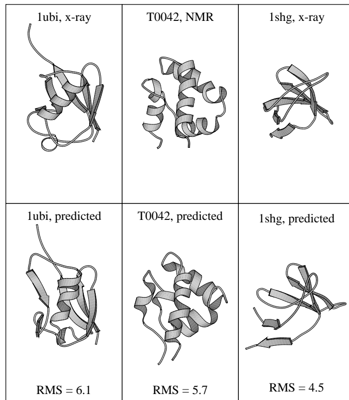
Figure 2. Comparison of the experimentally observed and predicted structure for the \alpha/\beta protein, 1ubi, the \alpha protein, target 42 of the CASP2 prediction competition, and the \beta protein 1shg, respectively. The top panel shows the experimental structures, while the lower panel shows the predicted structure. Also shown is the cRMSD in Å of all C \alpha atoms for the predicted conformation with respect to the native one.
